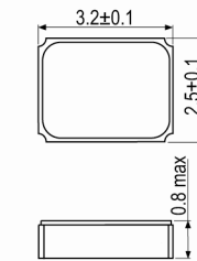
Outline (mm) -B = 4 pad
