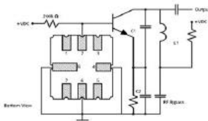
Typical Local Oscillator Application
