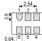
Underside View
